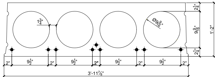
14" x 4'-0" HOLLOWCORE SLAB
